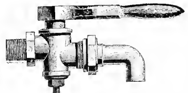
Fig. 3480. COMBINATION COCK FOR BAKER HEATERS.
